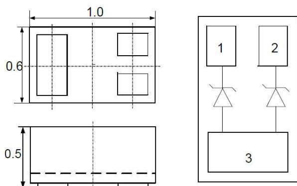
Package Dimensions
