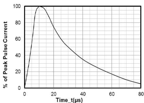
8 X 20 \mu\text{s} Pulse Waveform
