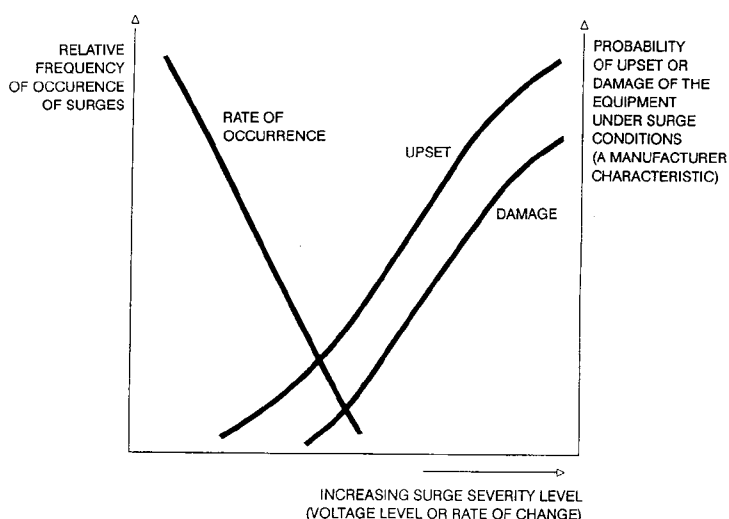
Figure 3—Probabilistic concept of surge immunity
