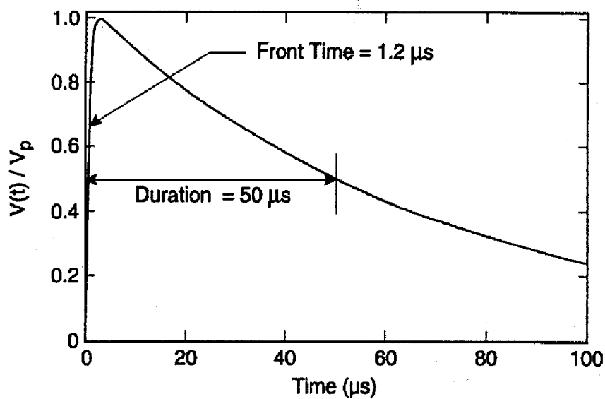
Figure 5—Combination Wave open-circuit voltage
