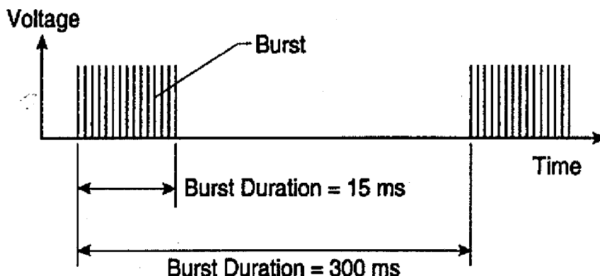
Figure 8—Pattern of EFT bursts
