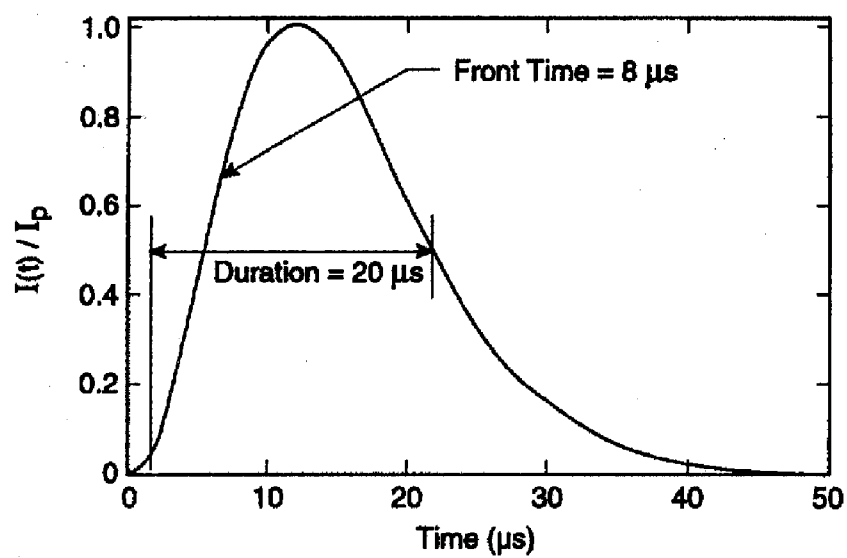
Figure 6—Combination Wave short-circuit current
