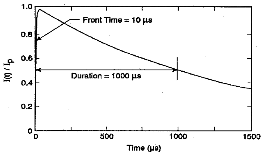
Figure 9—Waveform for the 10/1000 \mu s current surge
